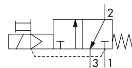
3/2-way function
