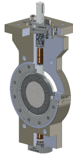
Fig. 2: Design of the control and shut-off valve type LTR 43-2
