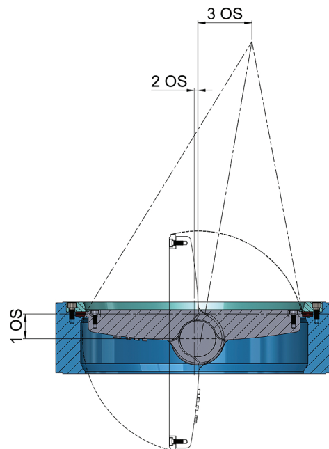
Fig. 3: Triple eccentricity
