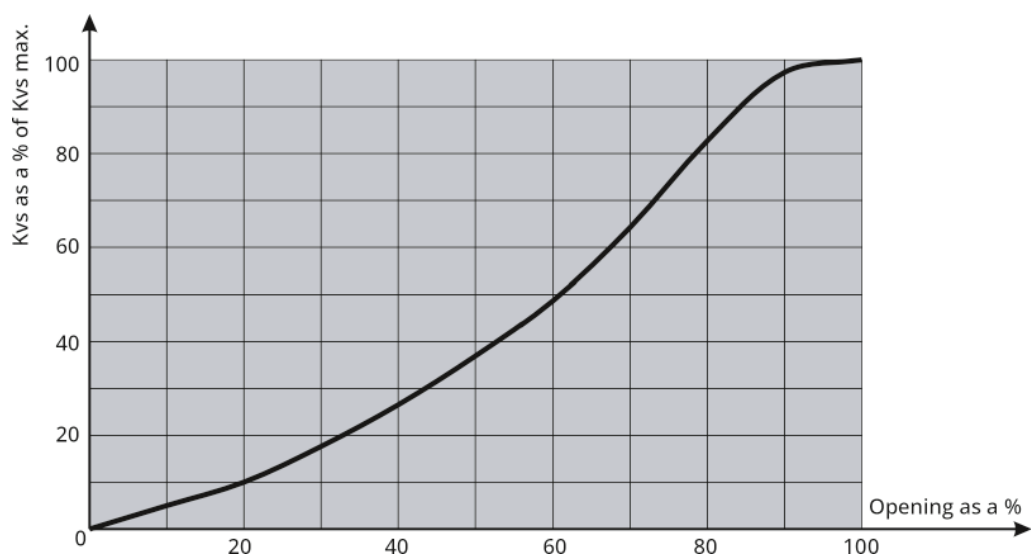
Fig. 6: Kvs-characteristic curve diagram
