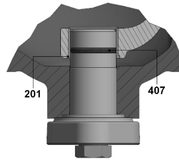
Trunnion Bearing Sealing 3)
