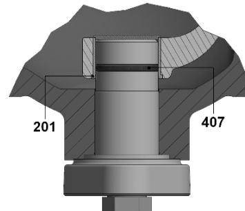
Trunnion Bearing Sealing 3)
